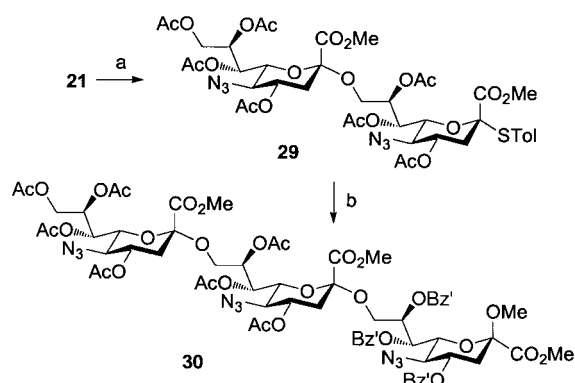
Scheme 6. a) 1) NaOMe, MeOH; 2) Ac 2 O, py, RT, 85% for both steps. b) 10 , NIS, TFOH, CH 3 CN, 3 Å MS, -40 °C, 1 h, 45%, \alpha .
